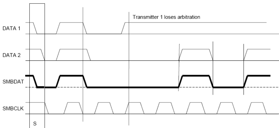
Figure 23-2 SMBus Arbitration
