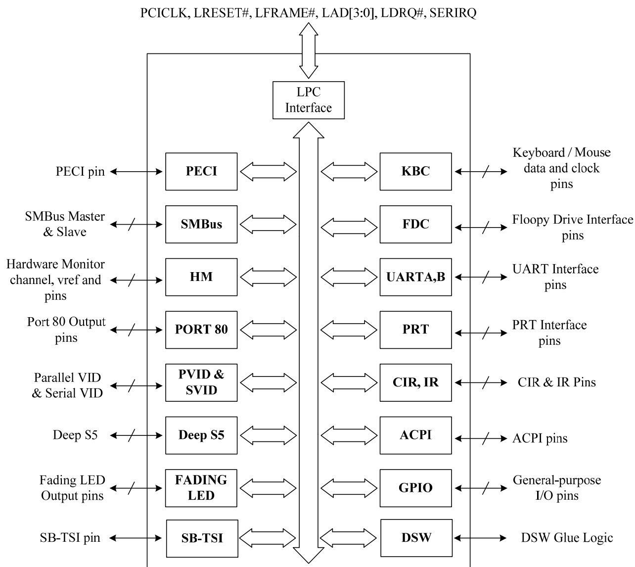
Figure 3-1 NCT6776F / NCT6776D Block Diagram
