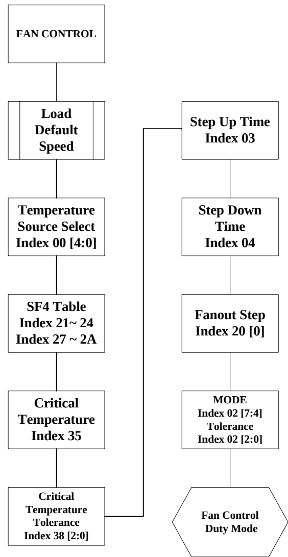
Figure 8-14 Fan Control Duty Mode Programming Flow
