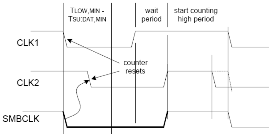
Figure 23-3 Clock synchronization
